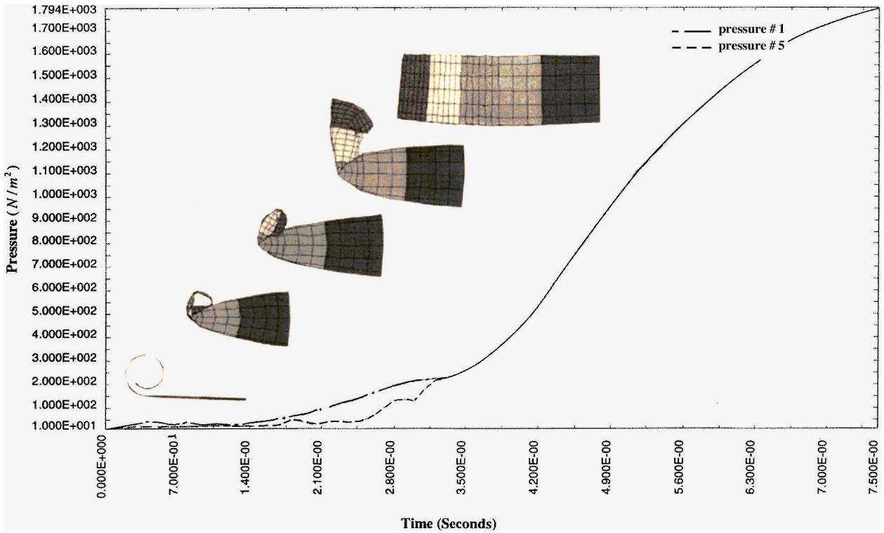
Fig. 3 Deployment of a rollout tube.
